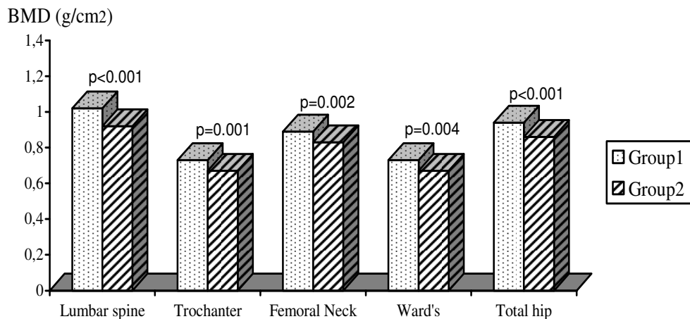
Figure 1 Means for BMD of various skeletal sites according to the timed get-up-and-go test (TGUGT). Abbreviations: BMD, bone mineral density. Group 1 was below the best cut-off (≤ 14.25 sec) and group 2 was above the best cut-off (>14.25 sec).
