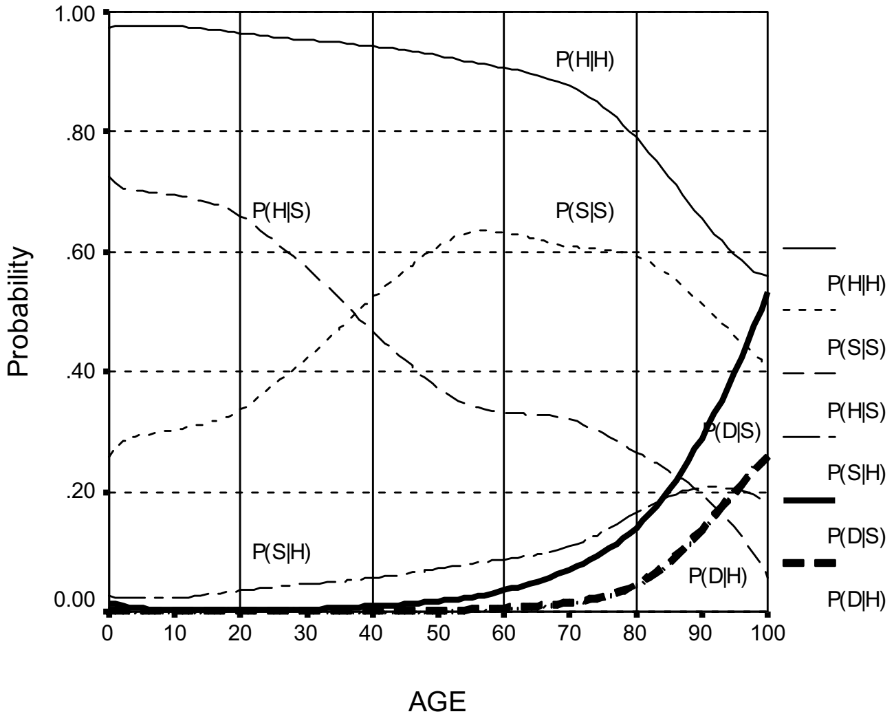
Figure 2 One-year Transition Probabilities.
