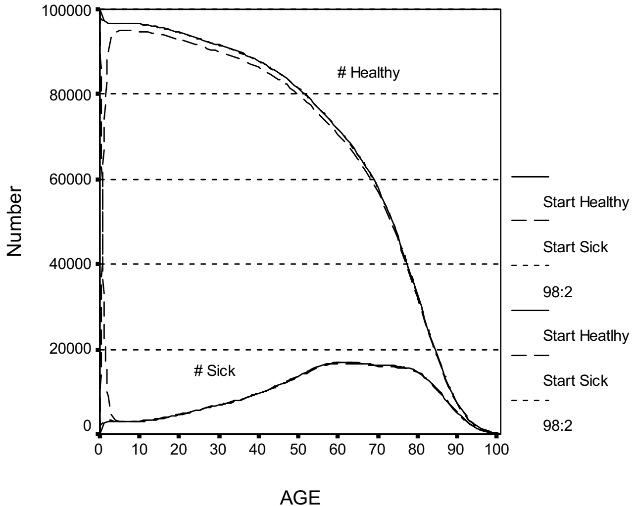
Figure 3 Estimated # of healthy and sick persons over time in Birth cohort (All healthy, All sick, or 98:2 ratio at Birth)*. *The topmost solid line is the number healthy when all were healthy at baseline, and the lower solid line is the number sick when all were healthy at baseline. The two dashed lines represent the number healthy and sick when all were sick at baseline. A third pair of dotted lines represent the number healthy and sick when 98% were healthy at baseline, but cannot be seen in this figure because they are essentially identical to the solid lines.
